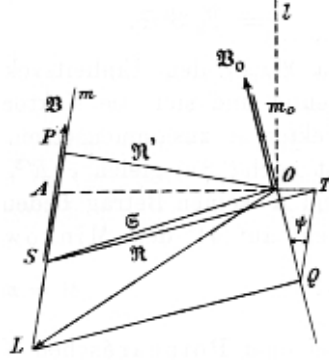
Figure 4: Sommerfeld's illustration of the two laws of gravitation (1910b, 687).
